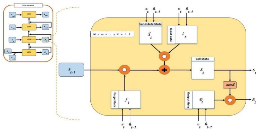
Figure 5. Schema of Long Short-Term Memory
