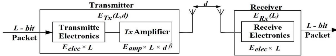
Figure 1. Radio Energy Dissipation Model.
