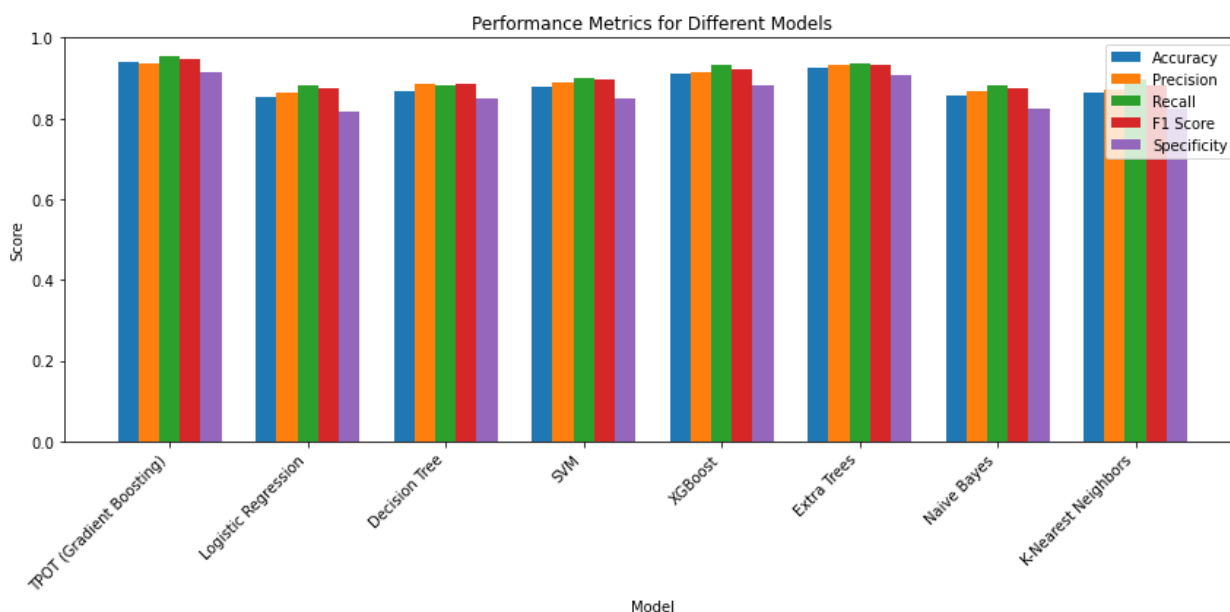
Figure 6. Visualization of Model Performance Across Evaluation Metrics
