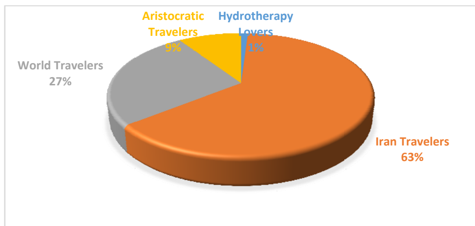
Figure3. Clusters' information
