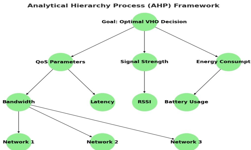
Figure 1. AHP Framework
